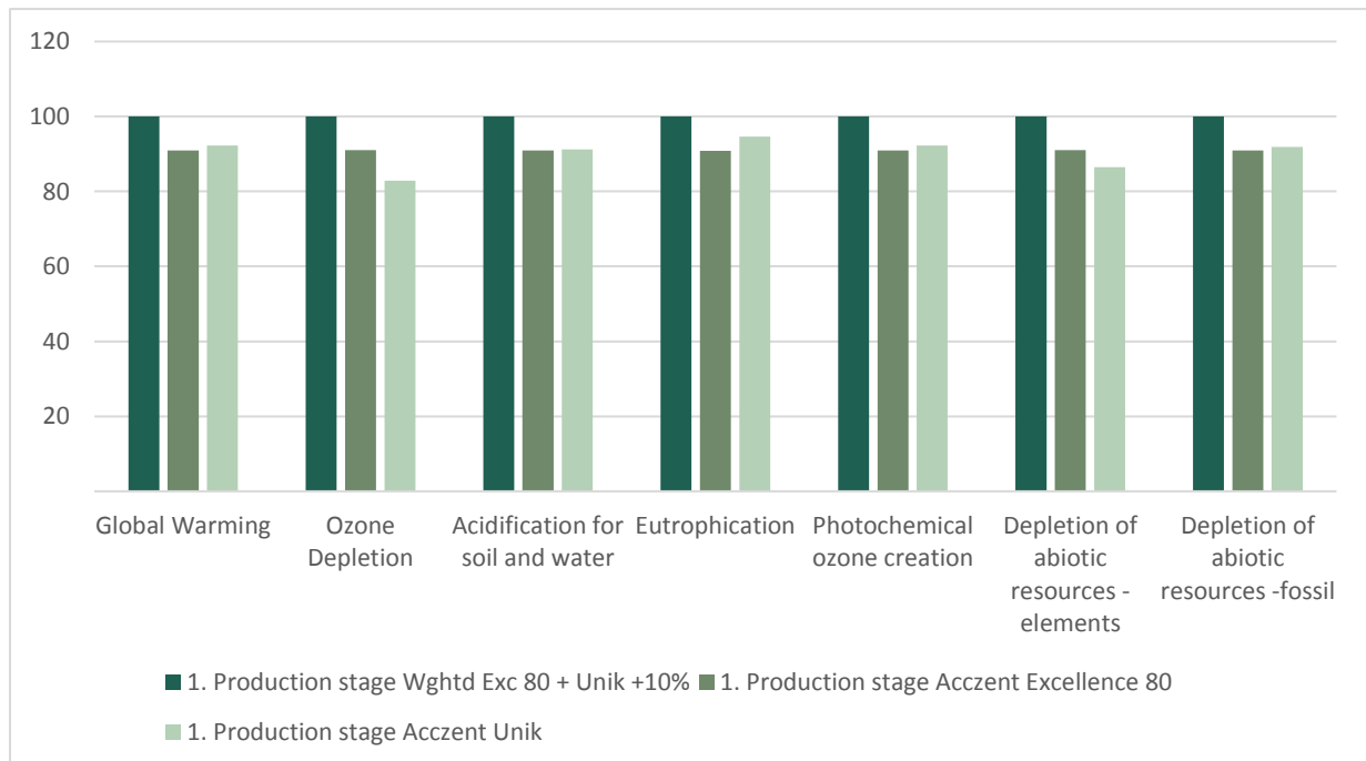
Figure 2: Comparison between Acczent Excellence 80, Acczent Unik and the average one (surface density between 3.05 and 3.25 kg/m 2 )
