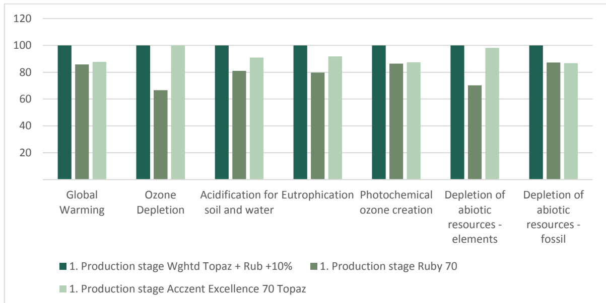
Figure 1: Comparison between Acczent Excellence 70 Topaz, Ruby 70 and the average one (surface density between 2.8 and 3.05 kg/m 2 )
